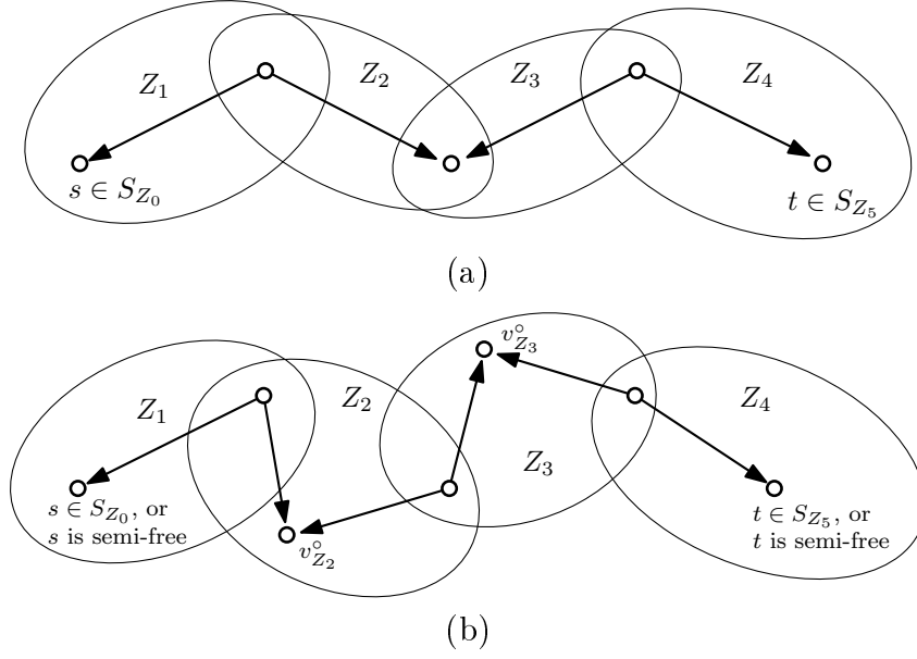
Figure 1: Examples of augmenting walks: (a) the case when there is no vertex of multiplicity two and (b) general case.
