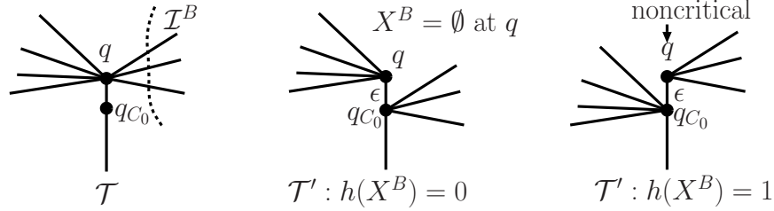
Figure 3: Tree modification I
