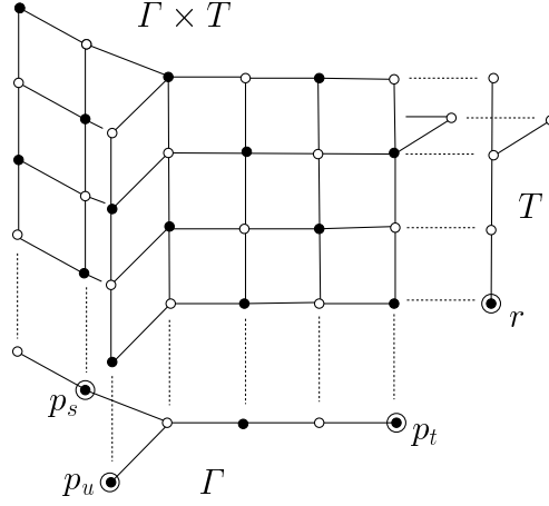
Figure 1: Product of two trees
