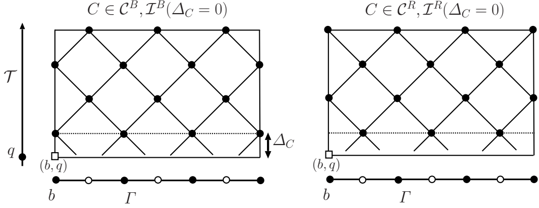
Figure 2: Drawing grids in C \times \bar{\Gamma} for (B) C \in \mathcal{C}^B \cup \mathcal{I}^B and (R) C \in \mathcal{C}^R \cup \mathcal{I}^R
