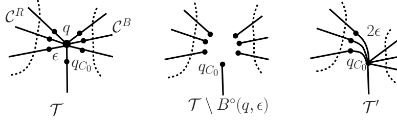
Figure 4: Tree modification II
