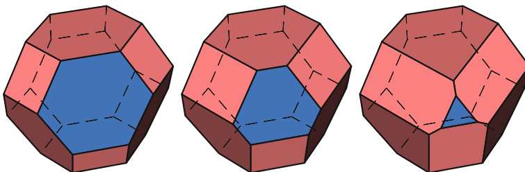
Fig. 1 Left an illustration of a g-polymatroid. Its vertices are all ordered distinct 3-tuples from \{0, 1, 2, 3\} . Its facet-defining inequalities are \binom{|S|}{2} \leq x(S) \leq 3|S| - \binom{|S|}{2} for each nonempty S \subsetneq [3] . The facet defined by x_1 + x_2 + x_3 \leq 6 is highlighted in blue. Center and right the polytopes obtained by increasing the right-hand side of the constraint x_1 + x_2 + x_3 \leq 6 to 6.5 and 7.2, respectively. The center polytope is still a g-polymatroid, but the rightmost is not
