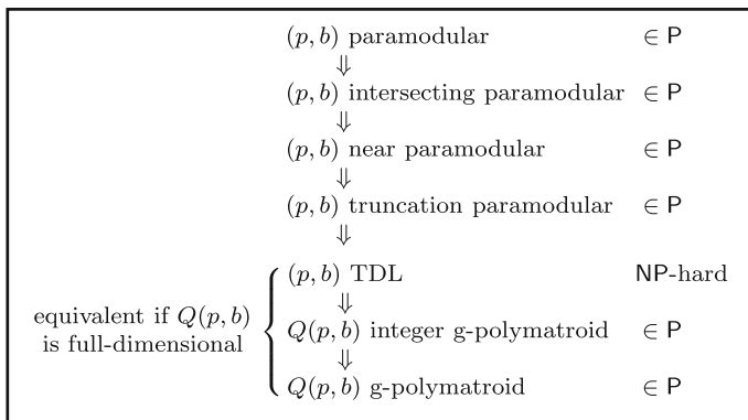
Fig. 2 Summarizing most of our results, where (p, b) is an integer-valued pair whose finite values are given explicitly as an input. The pre-existing notions of intersecting and near paramodularity are defined in Sects. 2.2 and 6, respectively
