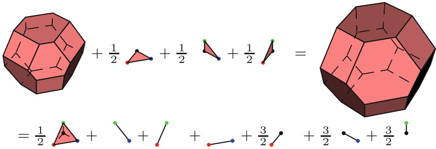
Fig. 3 Illustrating Theorem 1 for the g-polymatroid shown in the center of Fig. 1, where + indicates the Minkowski sum. The 4 coloured points denote the origin (black) and three standard unit basis vectors. The polyhedron in the right of Fig. 1 does not admit such a decomposition
